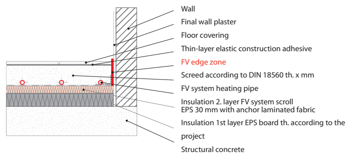
Picture no. 10: Fitting the FV edge strip
