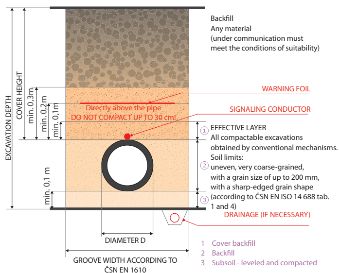
Scheme of laying FV HDPE 100 RC pipes in the excavation
