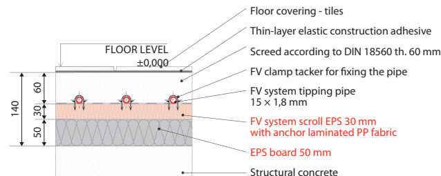
Picture no. 18: Recommended floor composition above heated rooms according to the recommendations of the ČSN EN 1264 standard thermal insulation resistance R = 2.00 m2K / W
