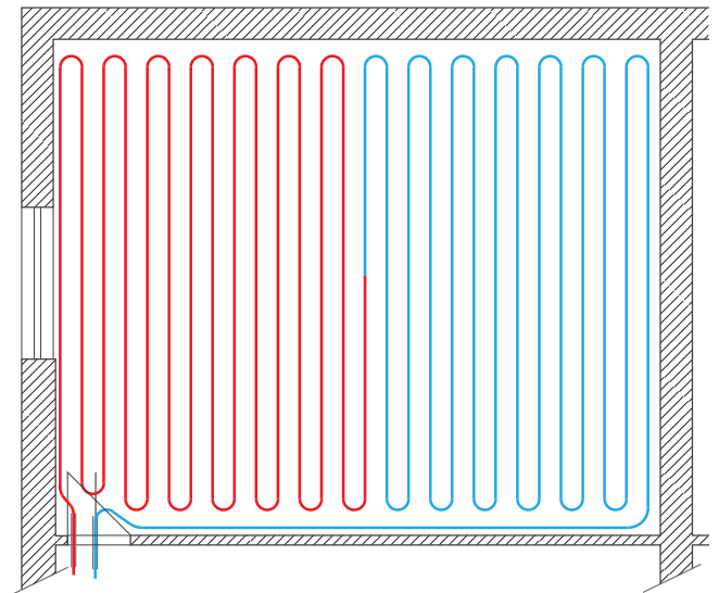
Picture no. 13: Meandering piping
