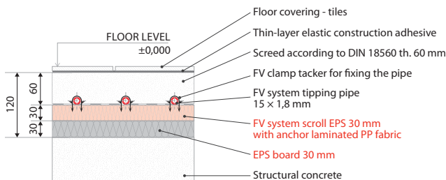
Picture no. 17: Recommended floor composition above heated rooms according to the recommendations of the ČSN EN 1264 standard thermal insulation resistance R = 1.25 m2K / W
