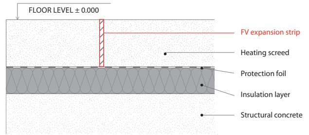
Picture no. 5: Expansion joint of heating screed when laying hard floor coverings (tiles, stone floor, laminate floor)
