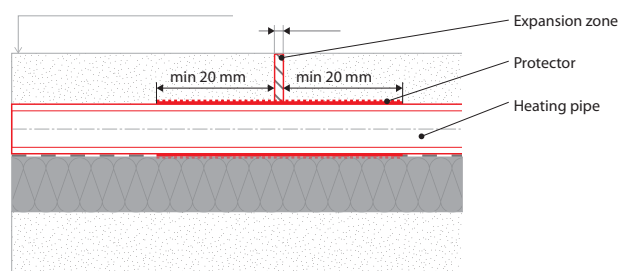
Picture no. 8: Protection of the heating pipe when passing through the expansion zone of the FV PE protector
