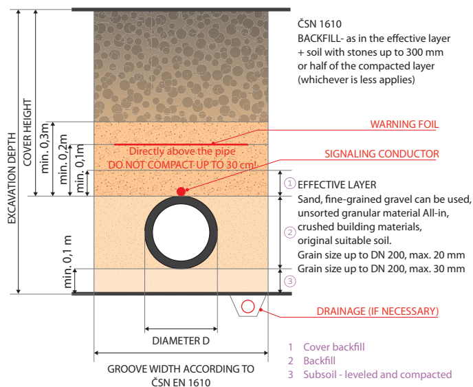
Scheme of laying FV HDPE 100 pipes in the excavation
