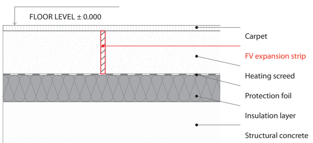
Picture no. 7: Expansion joint of heating screed when laying soft floor coverings (PVC, linoleum, carpet)
