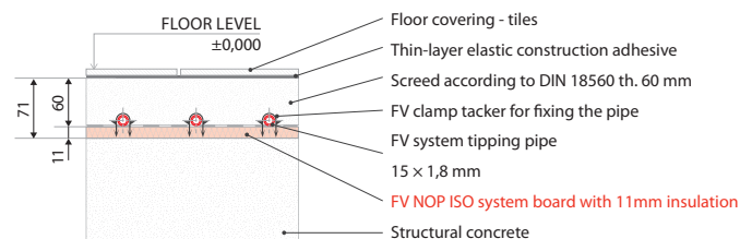
Picture no. 16: Recommended floor composition above heated rooms according to the recommendations of the ČSN EN 1264 standard thermal insulation resistance R = 0.75 m2K / W
