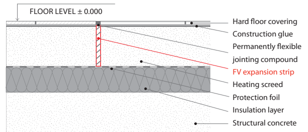
Picture no. 6: Expansion joint of heating screed when laying hard floor coverings with separating layer (tiles, stone floor, laminate floor)
